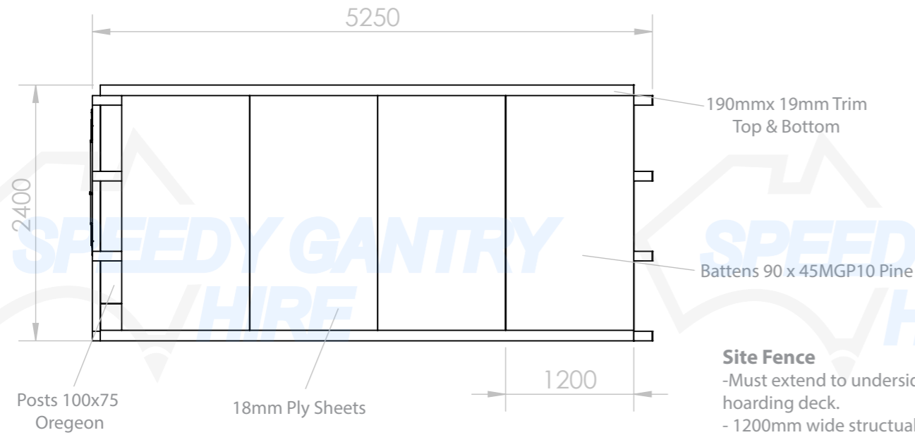
Front Elevation View
